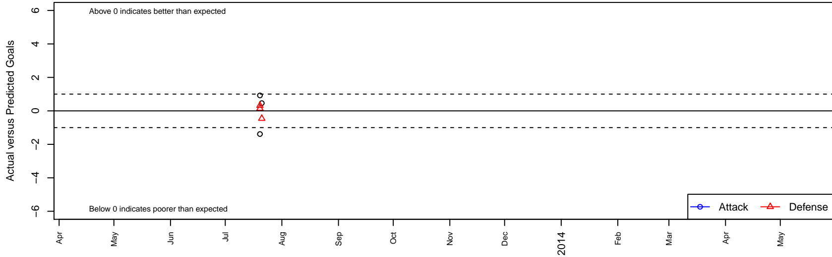
FC Golden State Black B00 Dots are actual minus expected GF (blue circles) and GA (red triangles). Blue line is smoothed change in attack strength. Red is smoothed change in defense strength.
